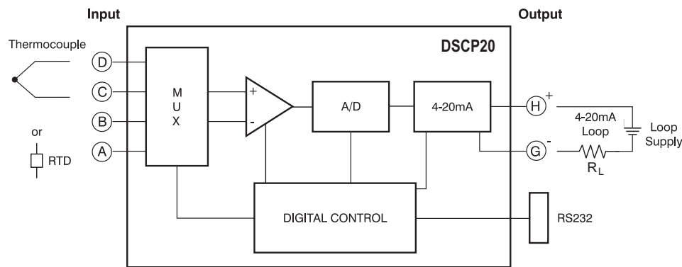
DSCP20 Block Diagram
