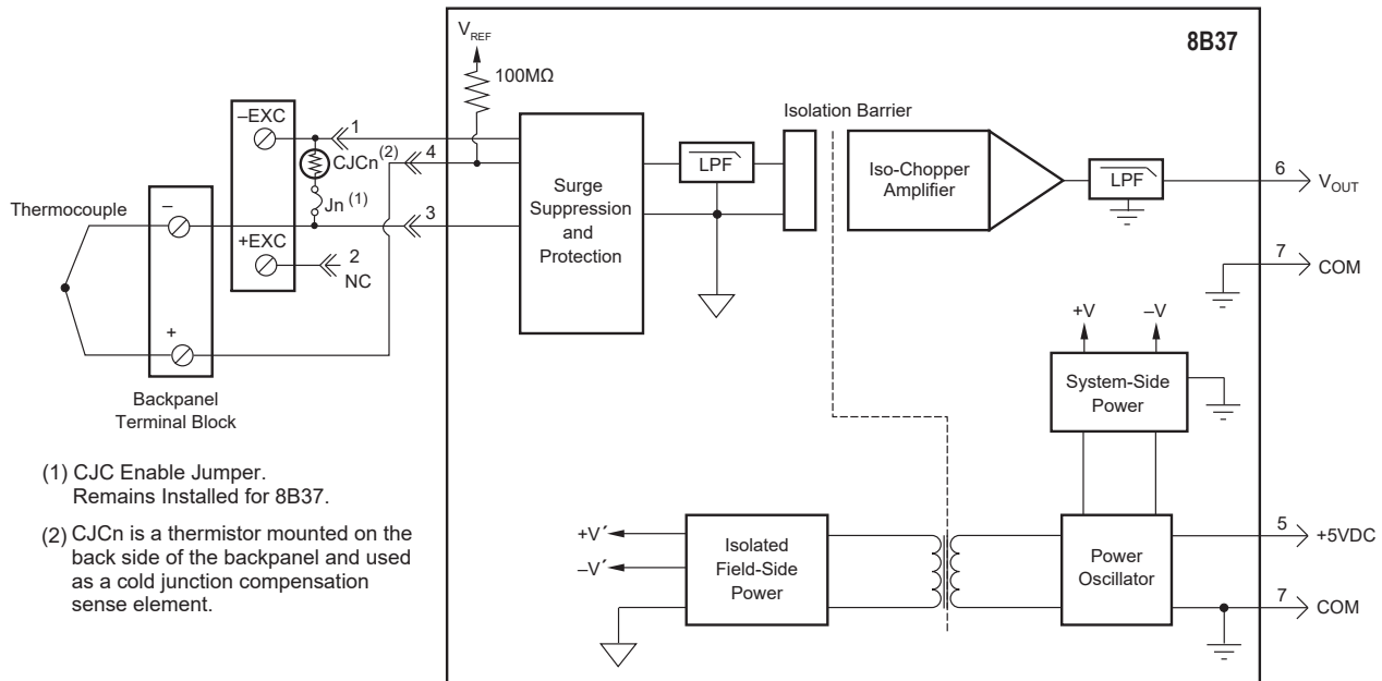
8B37 Block Diagram - For Module Dimensions and Pinouts. See Page 3-40
