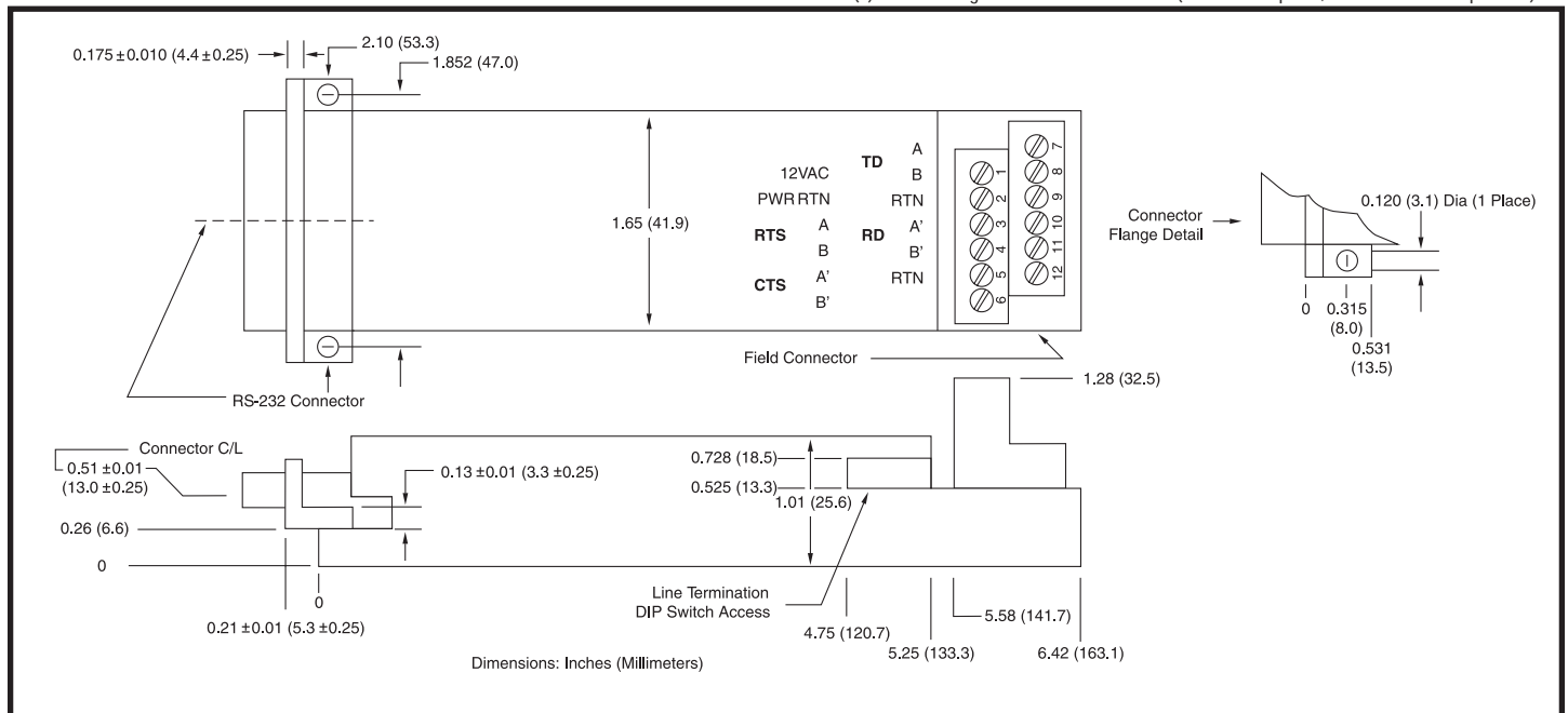
Figure 2: LDM485 Dimensions
